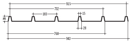
132 COPERNIT COPERALL 37 183 / 38
