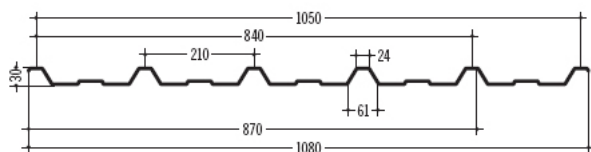
61 INCOFLUID 30/210/840 - 1050 210 / 30
