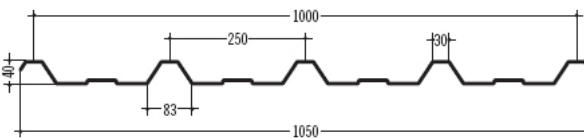
35 ISOLPACK R/W1000 250 / 40
