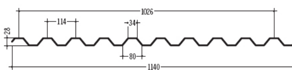
66 LANDINI H28/1140 114 / 28
