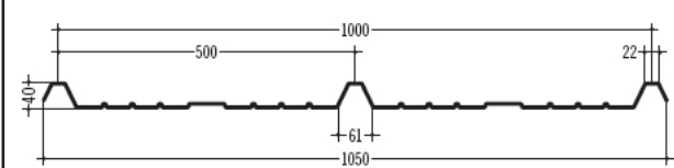
54 ISOPALCK DELTA 3 500 / 40
