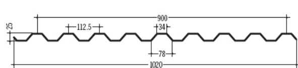
70 UNIMETAL GENUS 900 112.5 / 25
