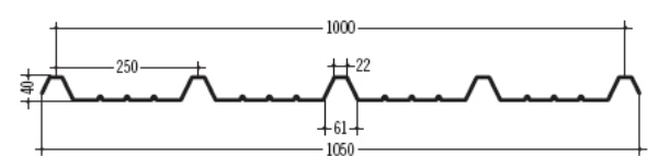
64 ISOLPACK DELTA 5 250 / 40
