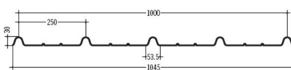
68 UNIMETAL GENUS 1000 250 / 30
