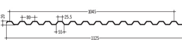
67 LANDINI H20 80 / 20
