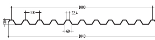
62 ALCAN GRECAL 30-100 100 / 30
