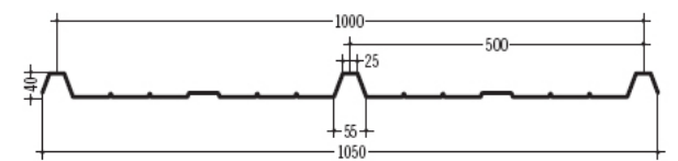
116 ISOPAN ISOTEGO 1000 500 / 40
