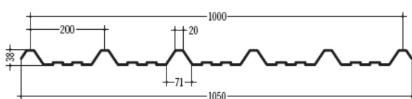
57 O.M.L. 6/38/1000 200 / 38
