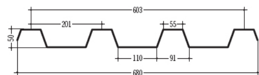
140 TECHNOIMES PROFILE 01 201 / 50
