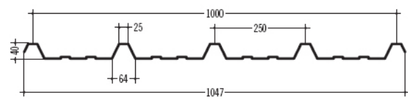
133 LANDINI H40/1047 250 / 40
