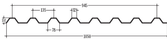
33 FIBROTUBI FIBRAL 135 / 32
